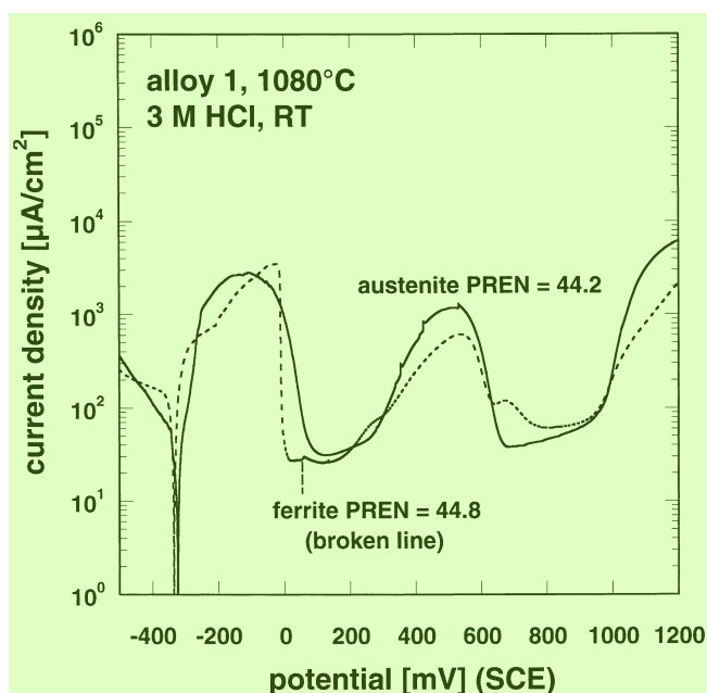
Fig. 8. Microelectrochemical polarisation curves of austenite and ferrite (in 3 M HCl at 23°C) of alloy 1 (solution annealed at 1080°C, one step).
