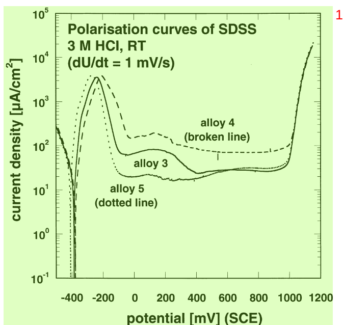
Fig. 4. Macroelectrochemical polarisation curves (in 3 M HCl at 23°C) of different SDSS. 2
