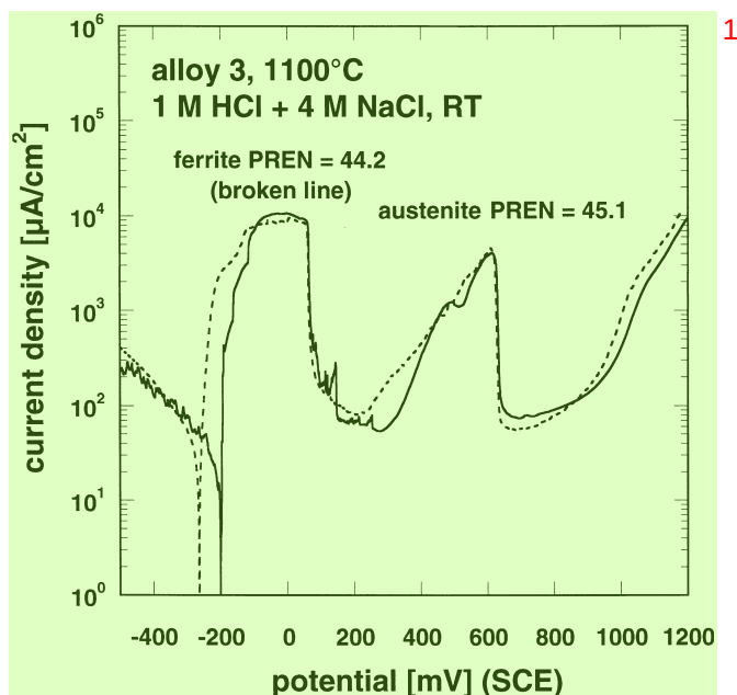
Fig. 5. Microelectrochemical polarisation curves of austenite and ferrite (in 1 M HCl + 4 M NaCl at 23°C) of alloy 3 (solution annealed at 1100°C, one step).
