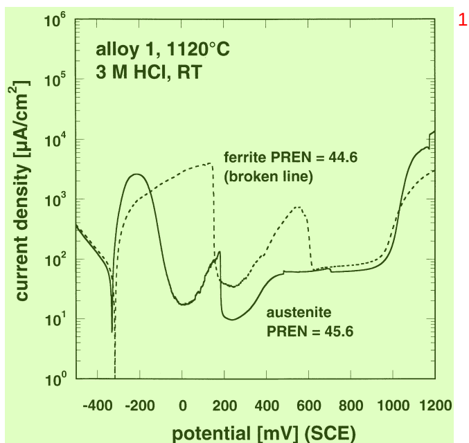
Fig. 9. Microelectrochemical polarisation curves of austenite and ferrite (in 3 M HCl at 23°C) of alloy 1 (solution annealed at 1120°, one step).
