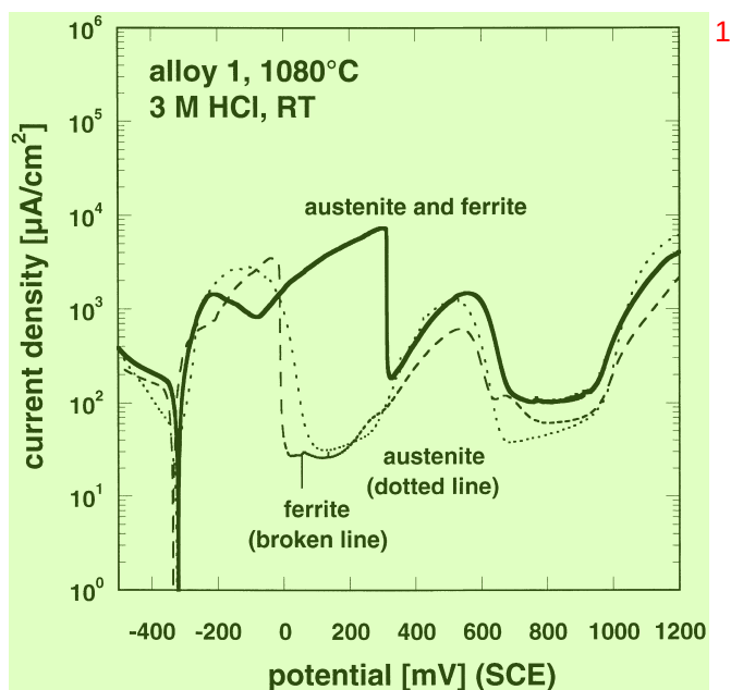
Fig. 13. Microelectrochemical polarisation curves of austenite, ferrite and the phase boundary (in 3 M HCl at 23°C) of alloy 1 (solution annealed at 1080°, one step). 1
