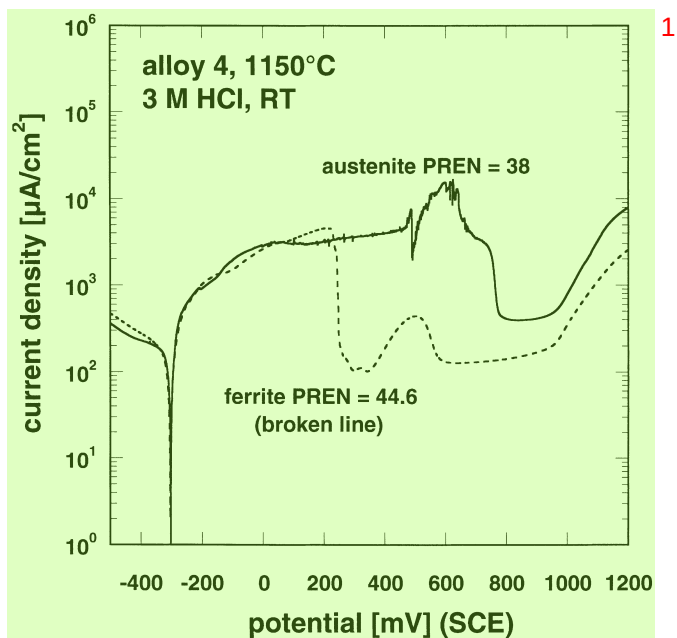
Fig. 6. Microelectrochemical polarisation curves of austenite and ferrite (in 3 M HCl at 23°C) of alloy 4 (solution annealed at 1150°C, one step).
