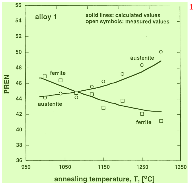
Fig. 2. PREN of the single phases as a function of the annealing temperature. 2
